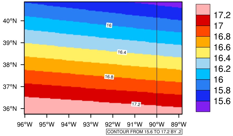
Yearly tasmx(c) In 2020-2029 GFDL-ESM2M RCP85 - Missouri
