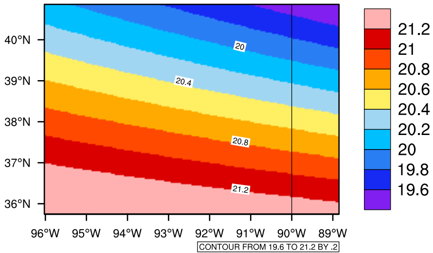
Yearly tasmax(c) In 2090-2099 GFDL-ESM2M RCP85 - Missouri
