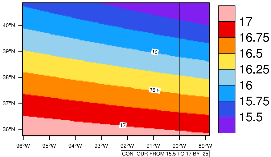
Yearly tasmax(c) In 1975-2005 GFDL-ESM2M historical - Missouri
