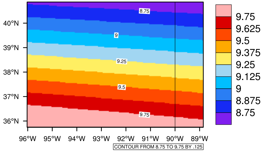
Yearly tasmin(c) In 2030-2039 GFDL-ESM2M RCP45 - Missouri
