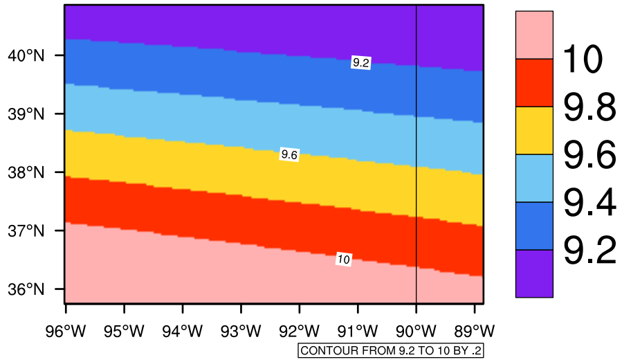
Yearly tasmin(c) In 2050-2059 GFDL-ESM2M RCP45 - Missouri
