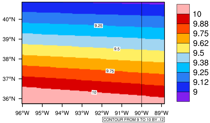
Yearly tasmin(c) In 2060-2069 GFDL-ESM2M RCP45 - Missouri
