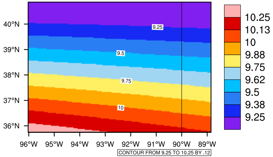
Yearly tasmin(c) In 2070-2079 GFDL-ESM2M RCP45 - Missouri
