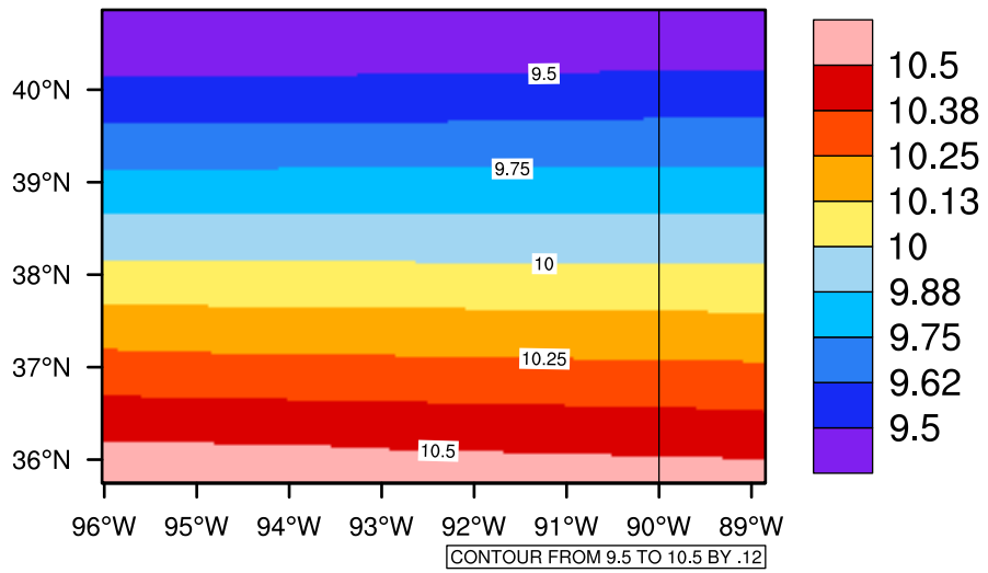
Yearly tasmin(c) In 2080-2089 GFDL-ESM2M RCP45 - Missouri
