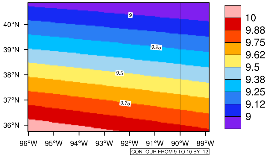
Yearly tasmin(c) In 2090-2099 GFDL-ESM2M RCP45 - Missouri
