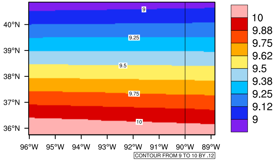
Yearly tasmin(c) In 2030-2039 GFDL-ESM2M RCP85 - Missouri
