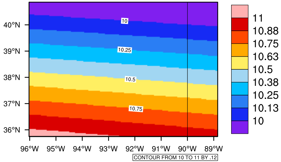
Yearly tasmin(c) In 2050-2059 GFDL-ESM2M RCP85 - Missouri
