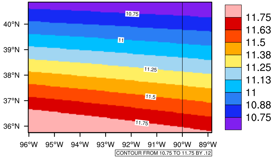
Yearly tasmin(c) In 2070-2079 GFDL-ESM2M RCP85 - Missouri
