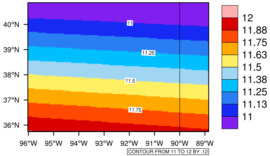
Yearly tasmin(c) In 2080-2089 GFDL-ESM2M RCP85 - Missouri
