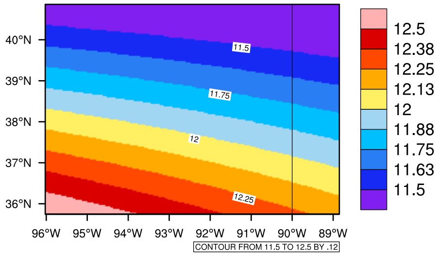
Yearly tasmin(c) In 2090-2099 GFDL-ESM2M RCP85 - Missouri
