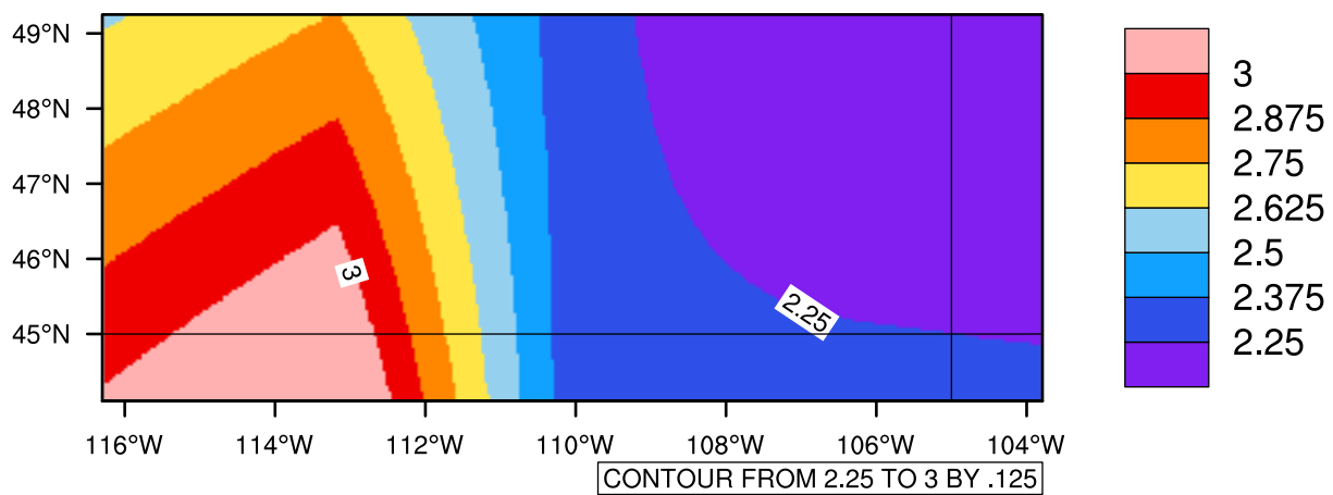
Yearly pr (mm/day) In 2030-2039 GFDL-ESM2M RCP45 - Montana
