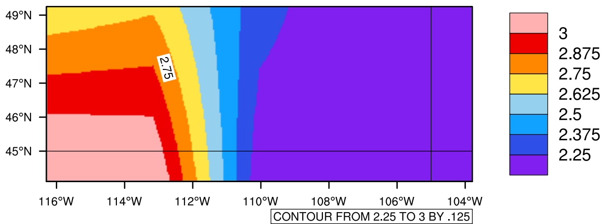
Yearly pr (mm/day) In 2040-2049 GFDL-ESM2M RCP45 - Montana
