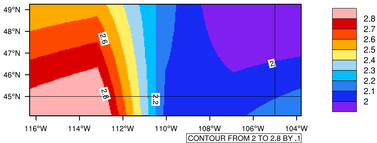
Yearly pr (mm/day) In 2060-2069 GFDL-ESM2M RCP45 - Montana
