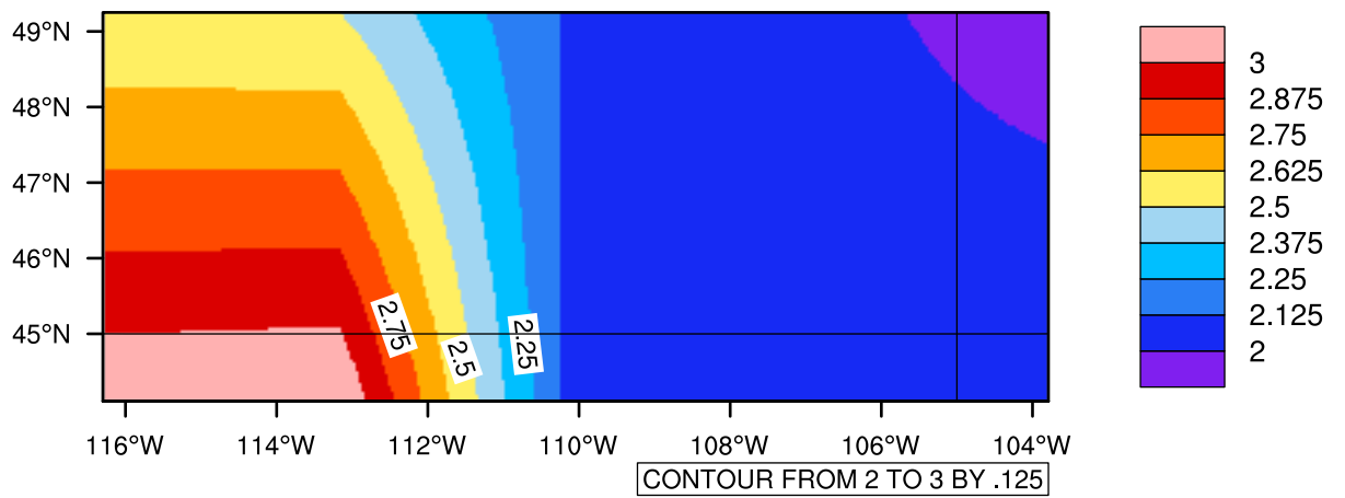
Yearly pr (mm/day) In 2080-2089 GFDL-ESM2M RCP45 - Montana
