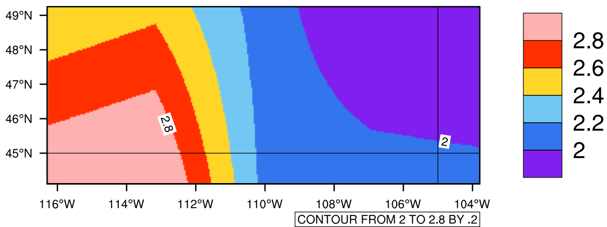
Yearly pr (mm/day) In 2020-2029 GFDL-ESM2M RCP85 - Montana
