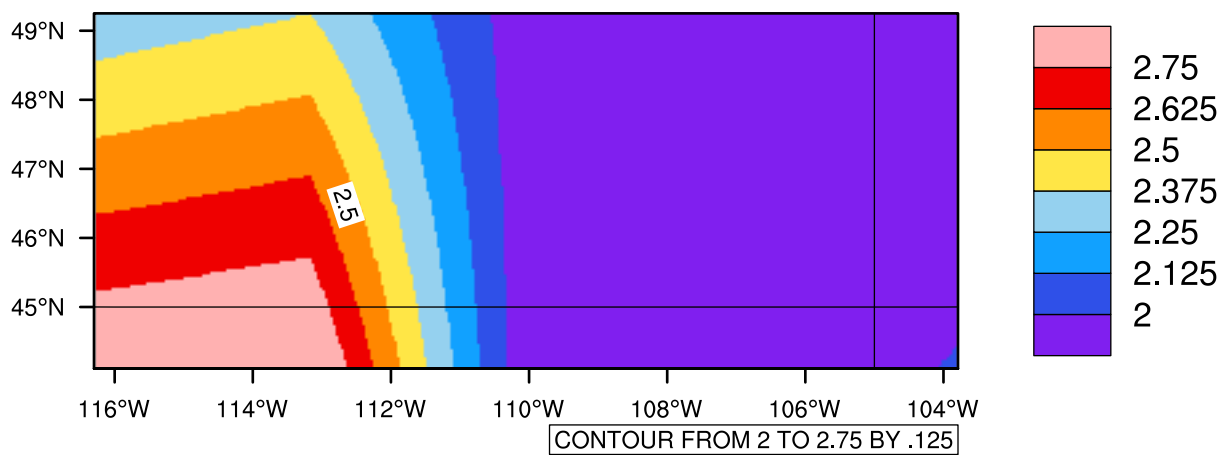
Yearly pr (mm/day) In 2030-2039 GFDL-ESM2M RCP85 - Montana
