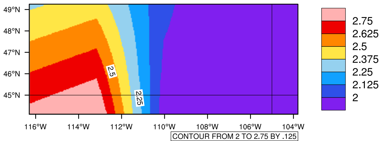
Yearly pr (mm/day) In 2040-2049 GFDL-ESM2M RCP85 - Montana
