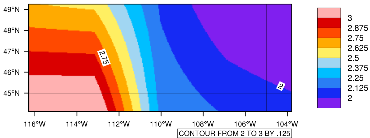
Yearly pr (mm/day) In 2060-2069 GFDL-ESM2M RCP85 - Montana
