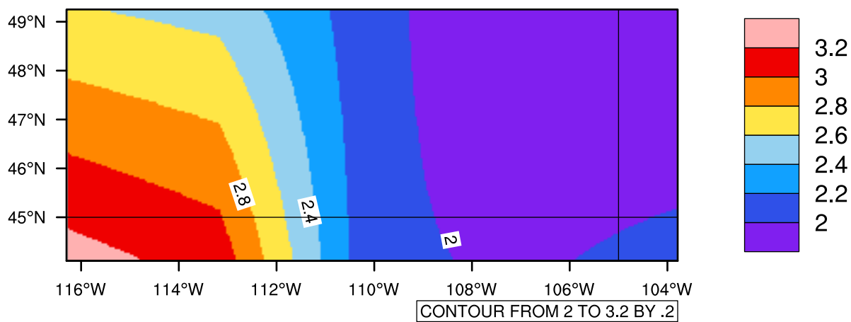
Yearly pr (mm/day) In 2070-2079 GFDL-ESM2M RCP85 - Montana
