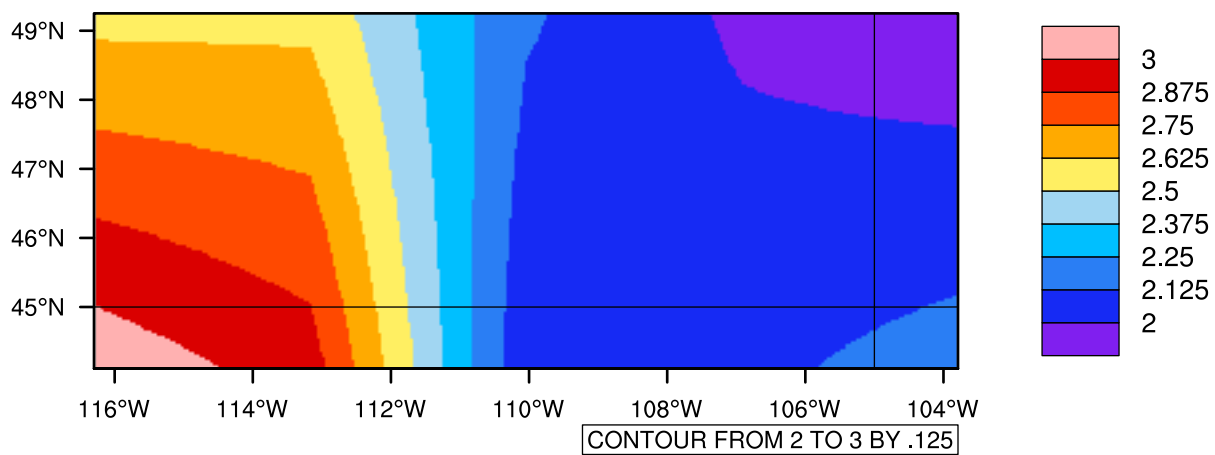
Yearly pr (mm/day) In 2080-2089 GFDL-ESM2M RCP85 - Montana
