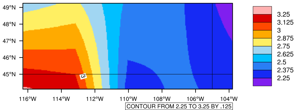
Yearly pr (mm/day) In 2090-2099 GFDL-ESM2M RCP85 - Montana
