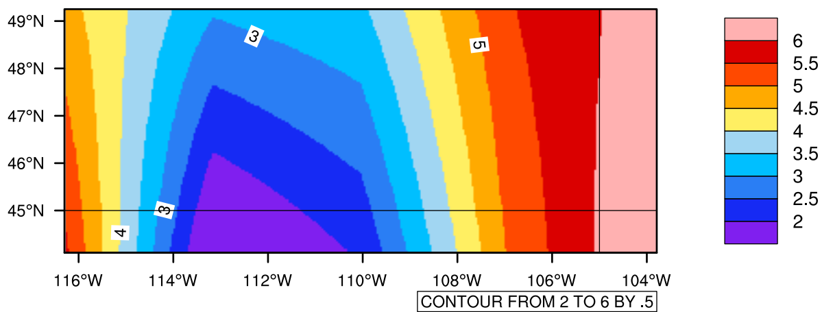
Yearly tas(c) In 2030-2039 GFDL-ESM2M RCP45 - Montana
