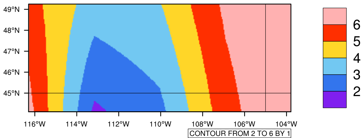
Yearly tas(c) In 2060-2069 GFDL-ESM2M RCP45 - Montana
