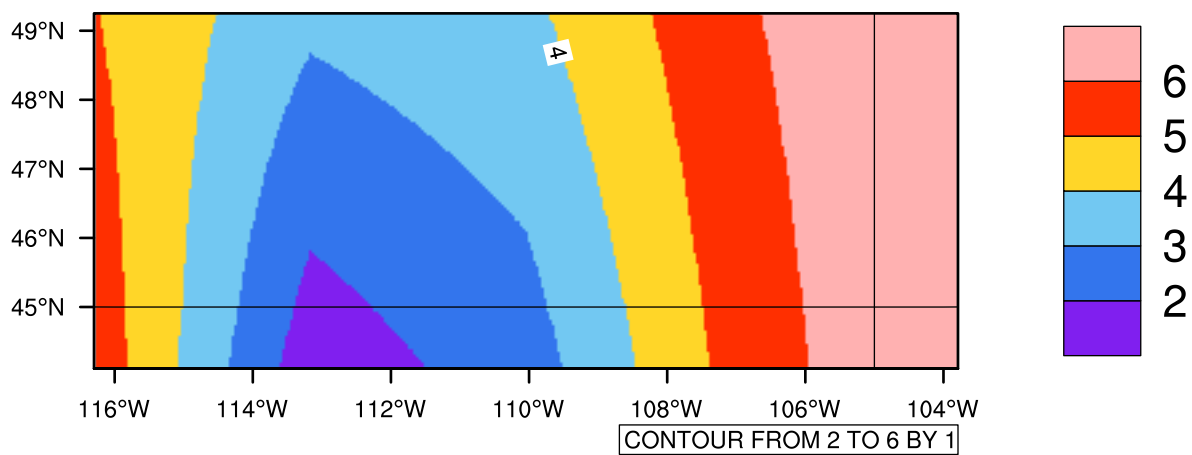
Yearly tas(c) In 2030-2039 GFDL-ESM2M RCP85 - Montana
