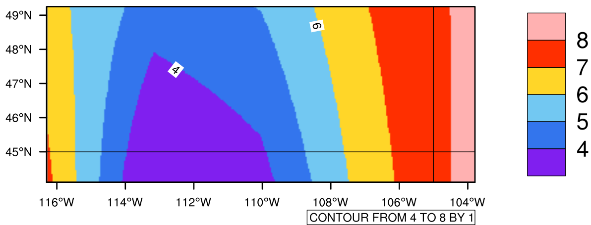
Yearly tas(c) In 2050-2059 GFDL-ESM2M RCP85 - Montana
