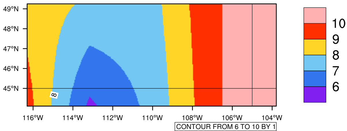
Yearly tasmax(c) In 2030-2039 GFDL-ESM2M RCP45 - Montana
