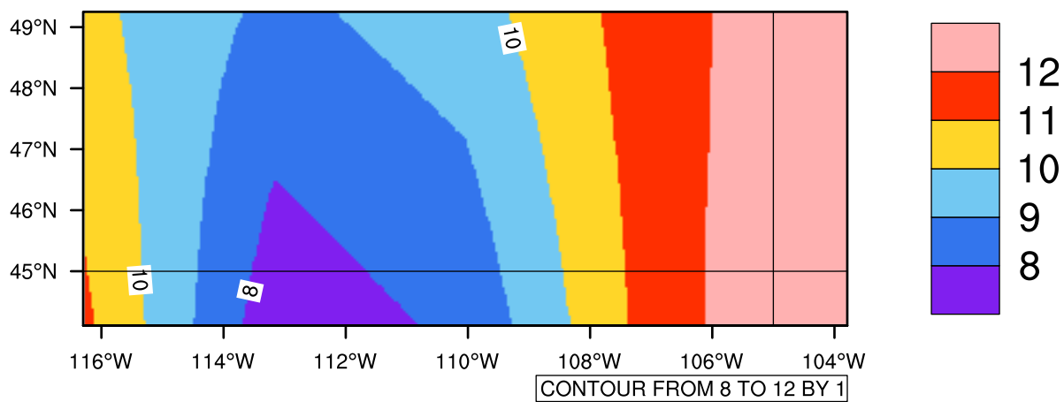
Yearly tasmax(c) In 2050-2059 GFDL-ESM2M RCP85 - Montana
