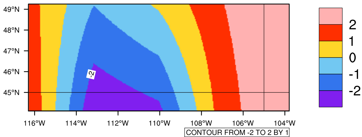
Yearly tasmin(c) In 2040-2049 GFDL-ESM2M RCP45 - Montana
