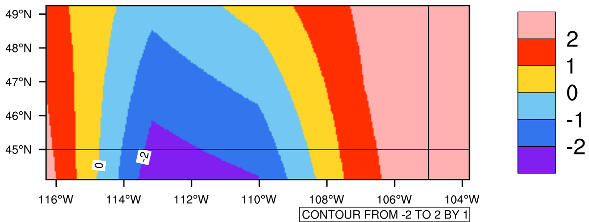
Yearly tasmin(c) In 2050-2059 GFDL-ESM2M RCP45 - Montana
