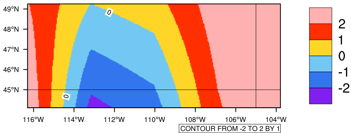
Yearly tasmin(c) In 2060-2069 GFDL-ESM2M RCP45 - Montana
