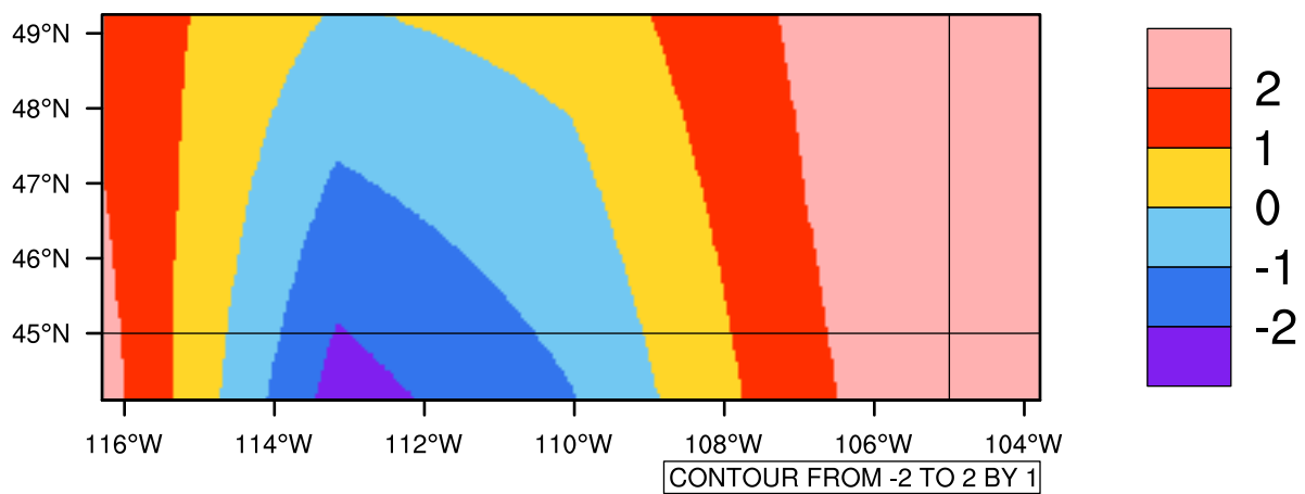
Yearly tasmin(c) In 2080-2089 GFDL-ESM2M RCP45 - Montana
