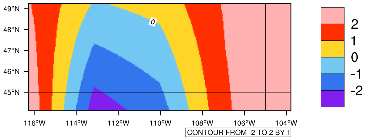
Yearly tasmin(c) In 2040-2049 GFDL-ESM2M RCP85 - Montana
