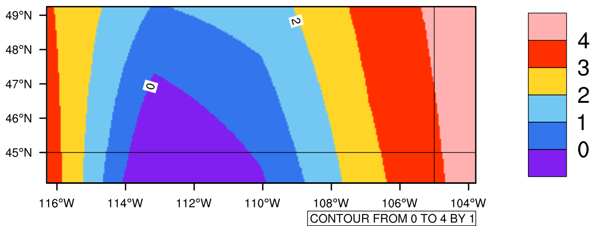
Yearly tasmin(c) In 2050-2059 GFDL-ESM2M RCP85 - Montana
