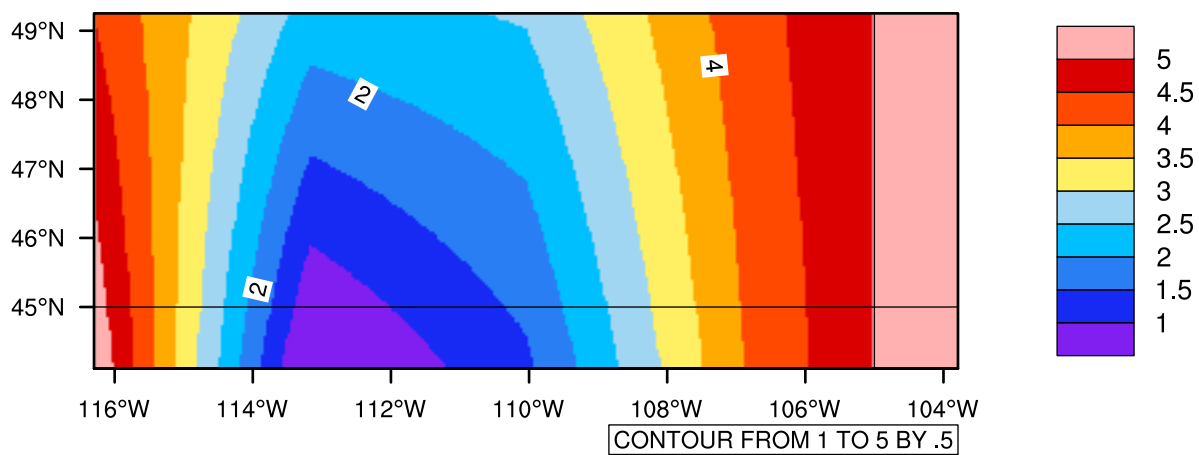
Yearly tasmin(c) In 2090-2099 GFDL-ESM2M RCP85 - Montana
