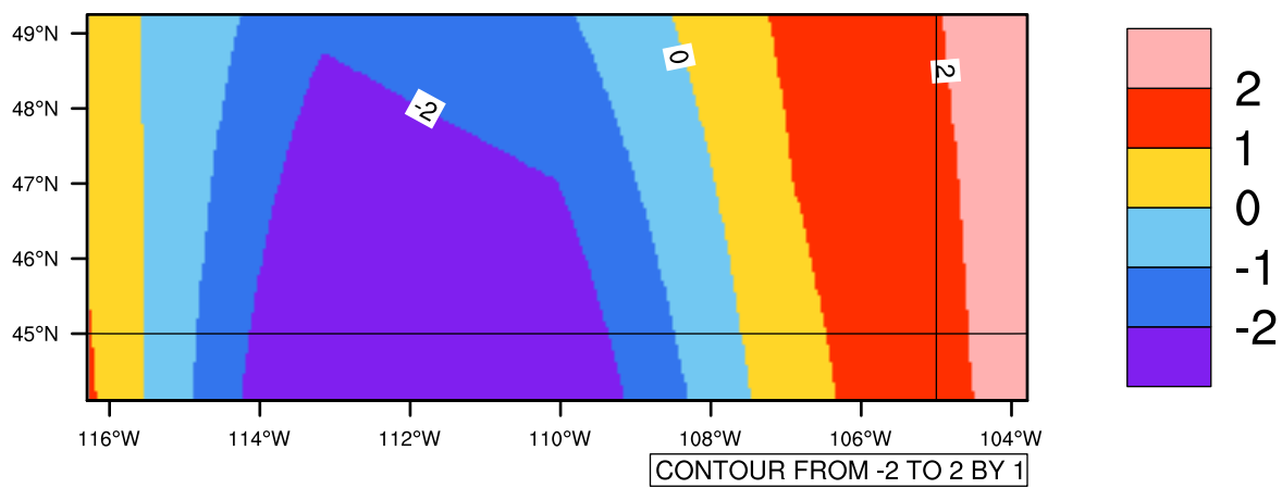
Yearly tasmin(c) In 1975-2005 GFDL-ESM2M historical - Montana
