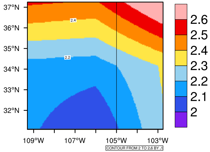
Yearly pr (mm/day) In 2020-2029 GFDL-ESM2M RCP45 - New Mexico
