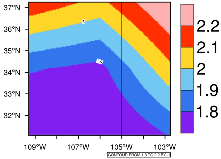
Yearly pr (mm/day) In 2070-2079 GFDL-ESM2M RCP85 - New Mexico
