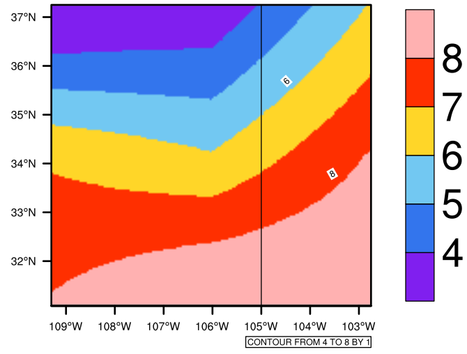
Yearly tasmin(c) In 1975-2005 GFDL-ESM2M historical - New Mexico
