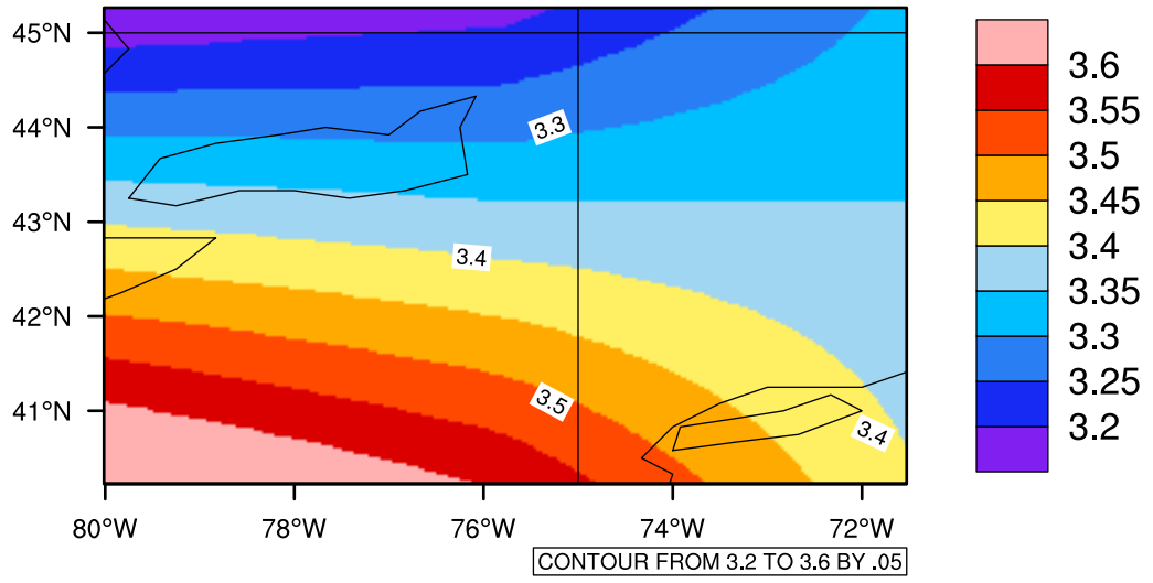
Yearly pr (mm/day) In 2050-2059 GFDL-ESM2M RCP45 - New York
