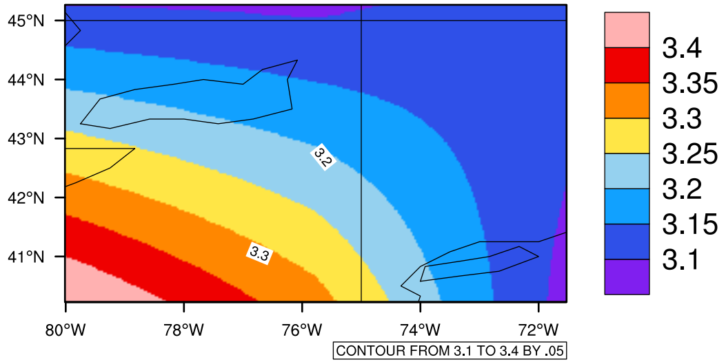
Yearly pr (mm/day) In 2070-2079 GFDL-ESM2M RCP45 - New York
