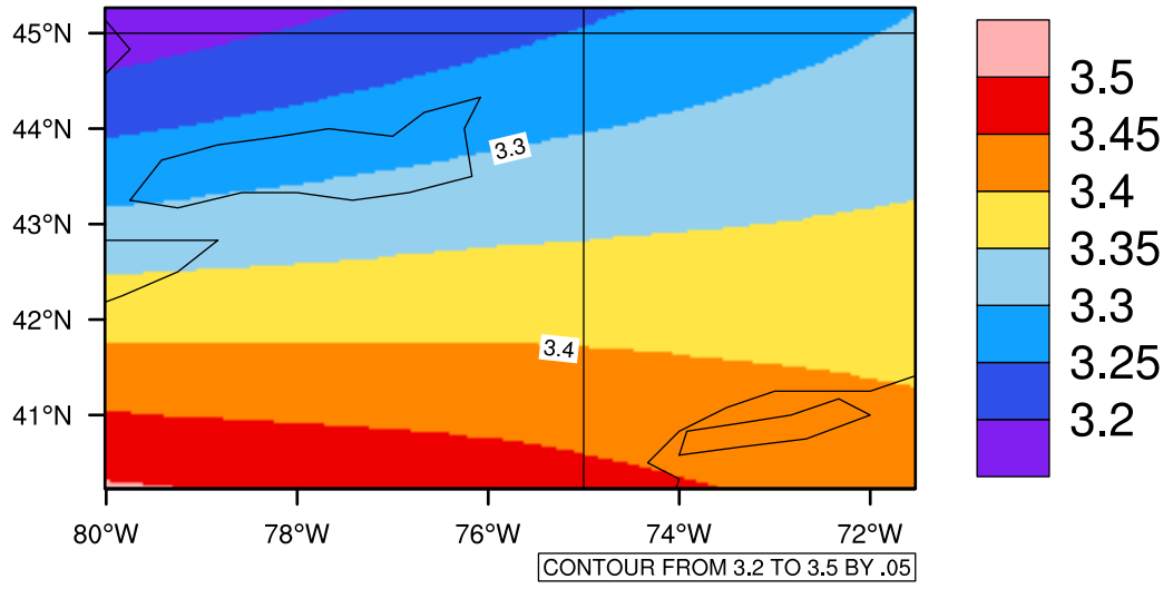
Yearly pr (mm/day) In 2090-2099 GFDL-ESM2M RCP45 - New York
