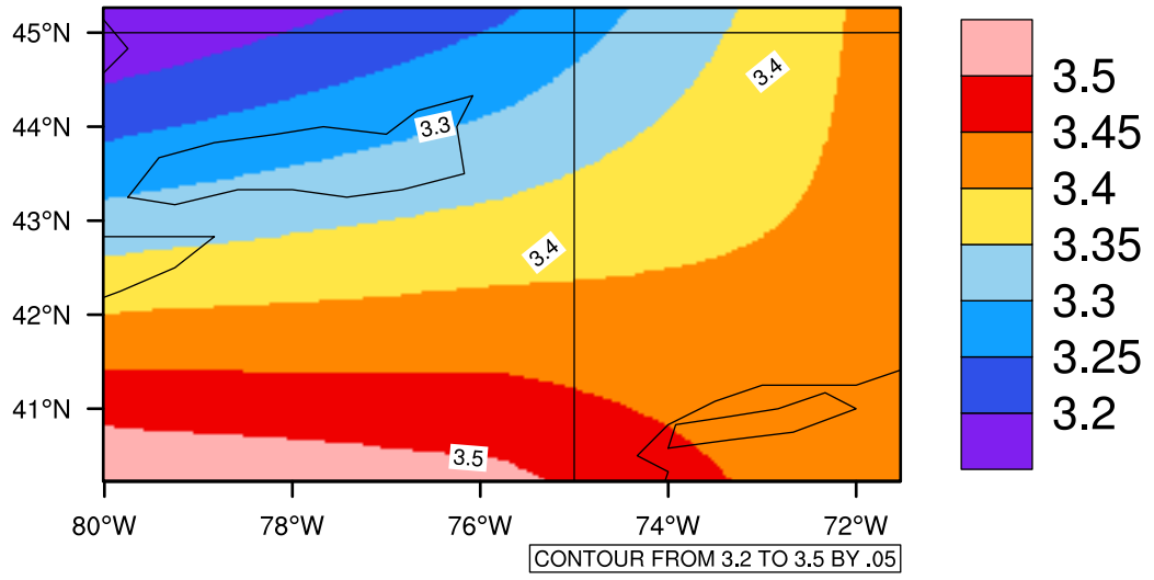
Yearly pr (mm/day) In 2070-2079 GFDL-ESM2M RCP85 - New York
