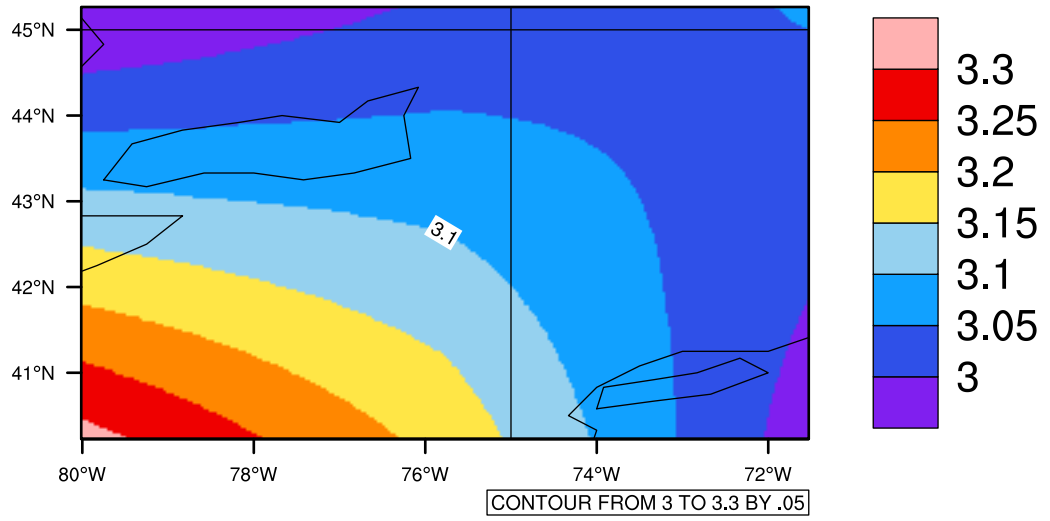
Yearly pr (mm/day) In 1975-2005 GFDL-ESM2M historical - New York
