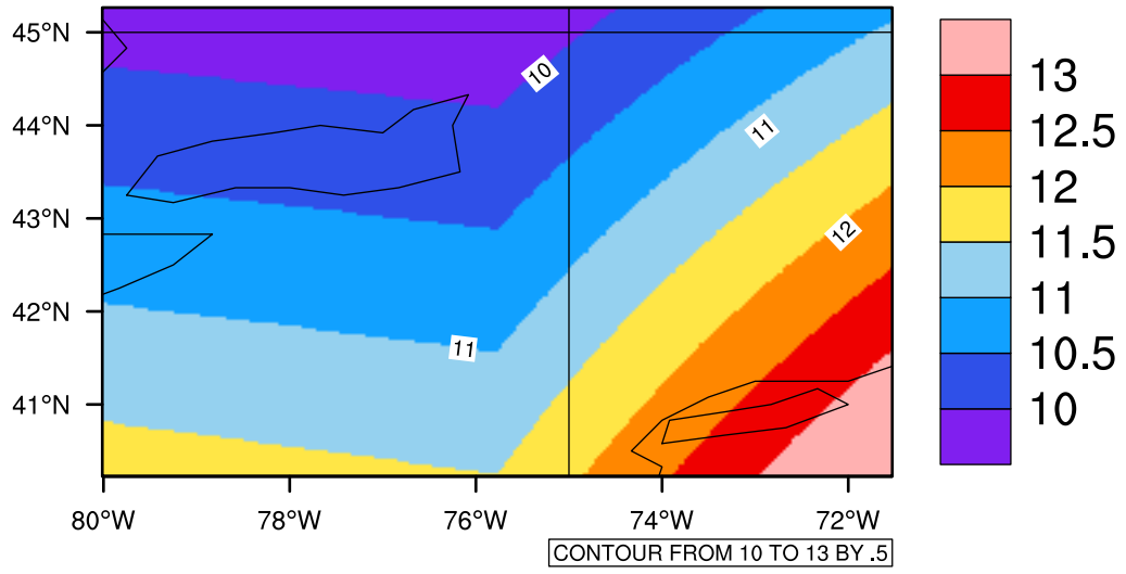
Yearly tasmax(c) In 2020-2029 GFDL-ESM2M RCP45 - New York
