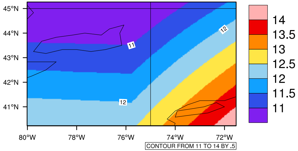
Yearly tasmax(c) In 2030-2039 GFDL-ESM2M RCP45 - New York
