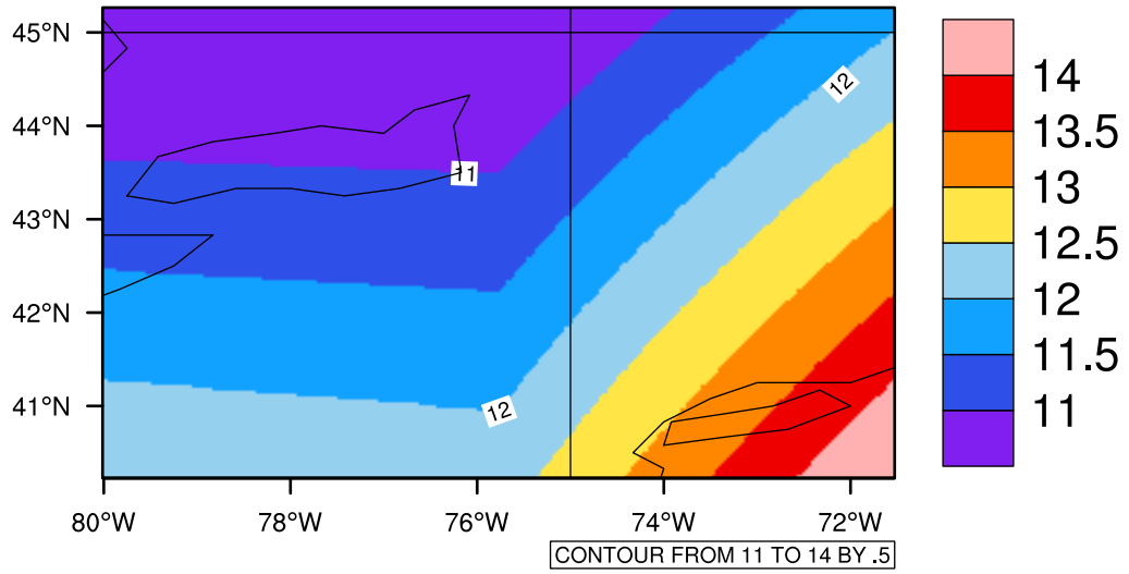
Yearly tasmax(c) In 2040-2049 GFDL-ESM2M RCP45 - New York
